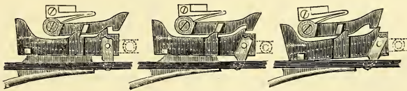
Jones' Single-trigger Mechanism.
